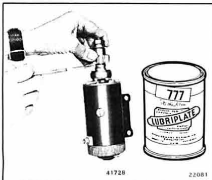
Figure 2-6. Starter Pinion Gear Shaft Helix
